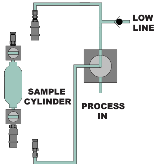
SEQUENCE 4 —Valve Position 1
