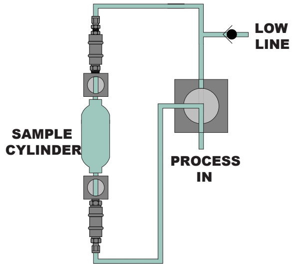
SEQUENCE 2 —Valve Position 2
