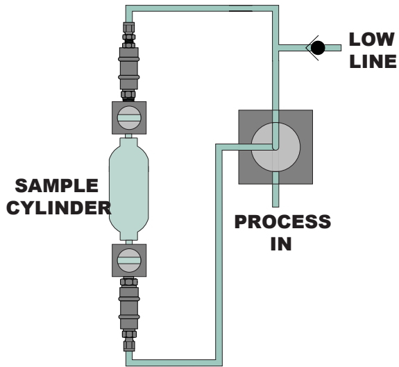
SEQUENCE 1 —Valve Position 1
