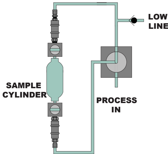
SEQUENCE 3 —Valve Position 1
